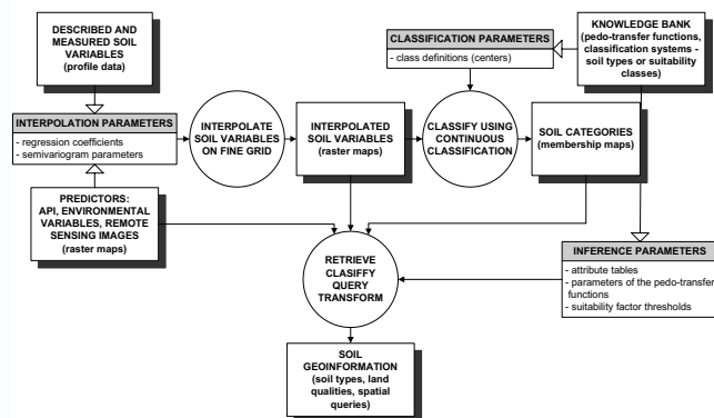
Fig. 2. Schematic flow of methodological steps used within the hybrid grid-based Soil Information System.
