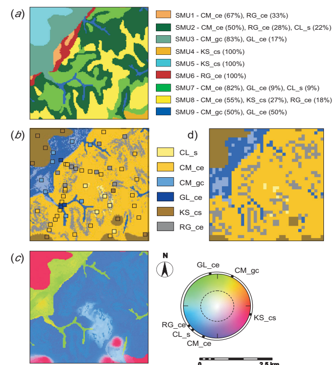
Fig. 4. Comparison of (a) the conventional soil map with compound composition of mapping units, (b) defuzzified (highest membership) map from the supervised fuzzy k-means classification with freely selected colours; (c) the continuous soil map with a circular legend and (d) down-scaled map to 100 m grid. CL_s – Siltic, Calcisols; CM_ce – Calcari-Eutric Cambisols; CM_gc – Gleyi-Calcari Cambisols; GL_ce – Calcari-Eutric Gleysols; KS_cs – Calci-Siltic Kastanozems and RG_ce – Calcari-Eutric Regosols.
