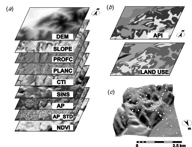
Fig. 3. Multi-source predictors: (a) auxiliary predictors terrain parameters and remote sensing data; (b) aerial photo-interpretation map (API) and land use map and (c) location of the 59 soil profile observations. DEM – elevation; SLOPE – slope gradient in %; PROF_C – profile curvature; PLANC – plan curvature; CTI – wetness index; SINS – slope insolation; AP – intensity of the aerial photo; AP_STD – standard deviation of the AP map and NDVI map derived from the Landsat 7 image.
