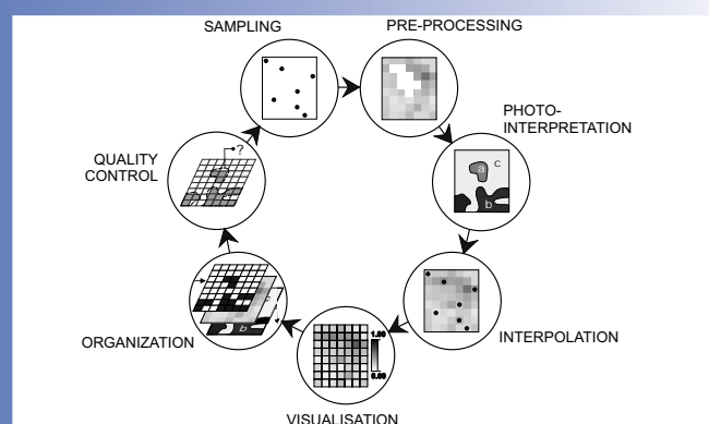
Fig. 1. Schematic outline of the topics discussed in the thesis. Note the circular structure, which symbolizes that the soil maps need to be periodically updated.
